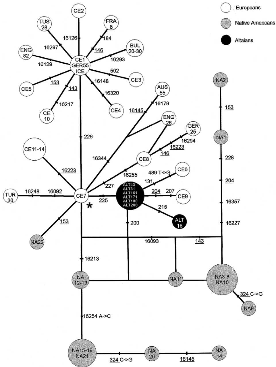
Figure 1 Reduced median network of haplogroup X mtDNAs, as defined by HVSI and HVSII variation. RFLP status of the sequences is known for American Indians (NA; Brown et al. 1998); for Altaians (ALT) from the present study; and for some Europeans (CE; Brown et al. 1998). The other European sequences—GER (Lutz et al. 1998), ENG (Piercy et al. 1993), TUS (Torrioni et al. 1996), FRA (Rousselet and Mangin 1998), BUL and TUR (Calafell et al. 1996), AUS (Parson et al. 1998), and ICE (Helgason et al. 2000)—were assumed, on the basis of their HVSI and HVSII sequences, to belong to haplogroup X. Sample origin is indicated by the scheme (see key). mtDNA types are represented by circles, with areas proportional to number of individuals. Lines are labeled by HVSI and HVSII mutations. Nucleotide variants correspond to transitions, whereas transversions are further specified. The insertions/deletions, as well as variations of C's in the unstable regions between nucleotide positions 16182–16193 and 309–315 were not included. The node marked with an asterisk (*) matches the haplogroup X basic motif: –1715c, +14465s, 16189C, 16223T, 16278T, +16517e/16519C, 153A, 195C, and 225A. The restriction site changes indicated by their enzyme letter code listed in table 1. Underlining indicates nucleotide positions that have mutated more than once, and reticulations indicate ambiguity in the topology. Parallel lines in a reticulation represent the same mutation.
